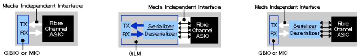
Figure 4.3 Flexible use of gigabit copper or fiber optics
